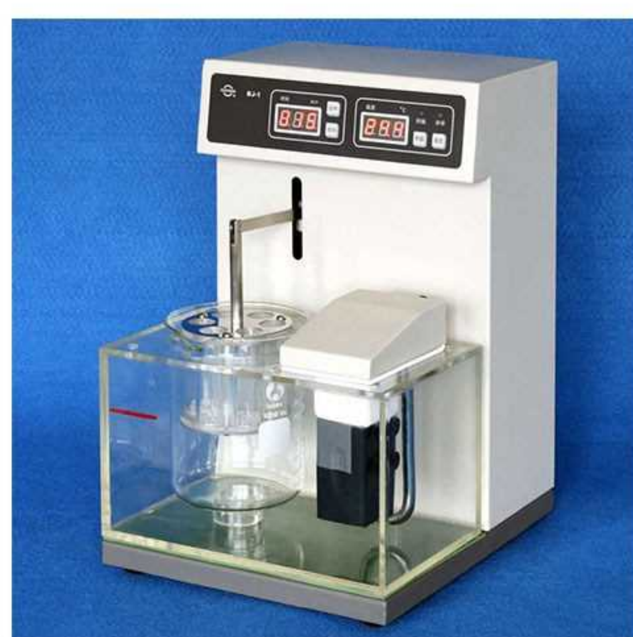
Disintegration Tester
